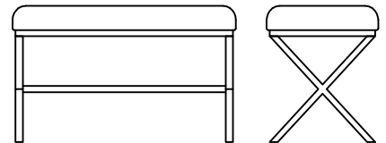
LUGGAGE BENCH 36"W x 18"D x 22"H
