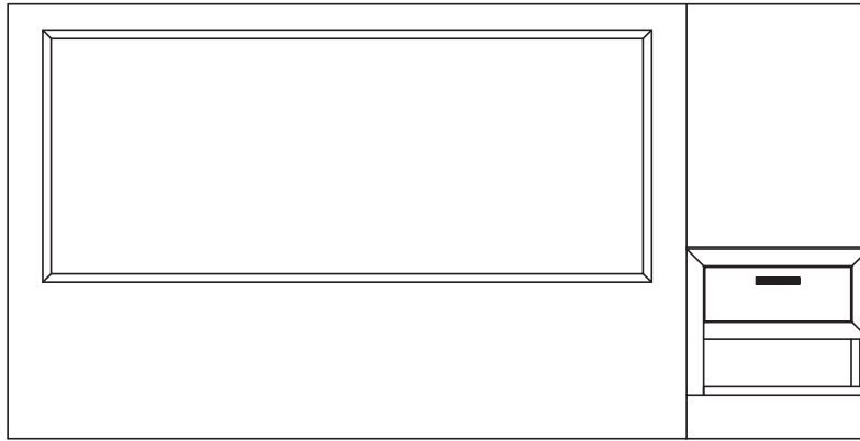
King Headboard with Nightstand (K/D) 99"W x 19 3/8"D x 50"H
